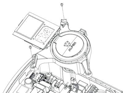
Figure 6: Detach subframe
