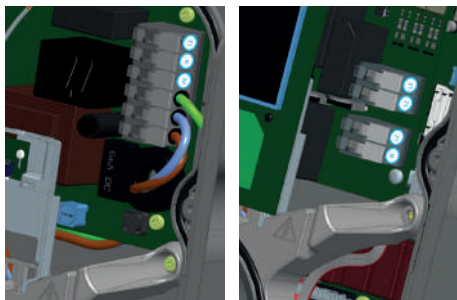
Figure 7a and 7b: Attaching individual charging cable wires on S-line 1 phase models (left) and S-line 3 phase & Pro-line models (right).
