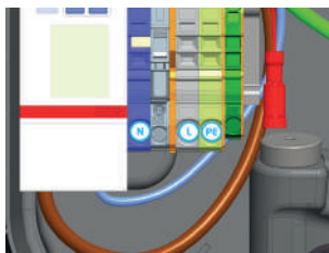
Figure 8a: Connection clamps power and Control Pilot (CP) connector for the charging cable (red) to S-line 1 phase.
